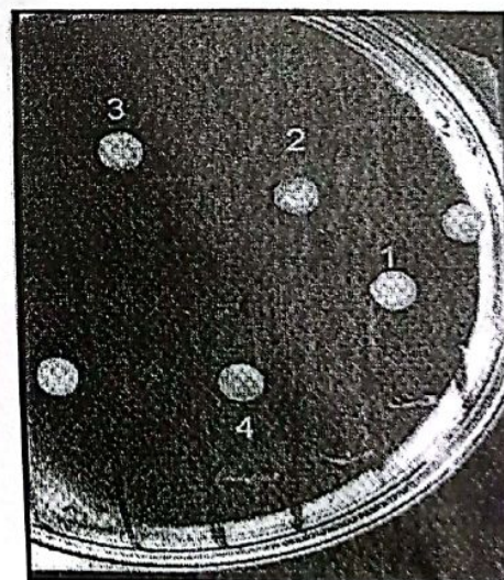
Photo. (2): Shows digitonin sensitivity test results. Colonies 1, 2 and 3 were sensitive to digitonin ( Mycoplasma and Ureaplasma ), while colony 4 was resistant ( Acholeplasma ).
