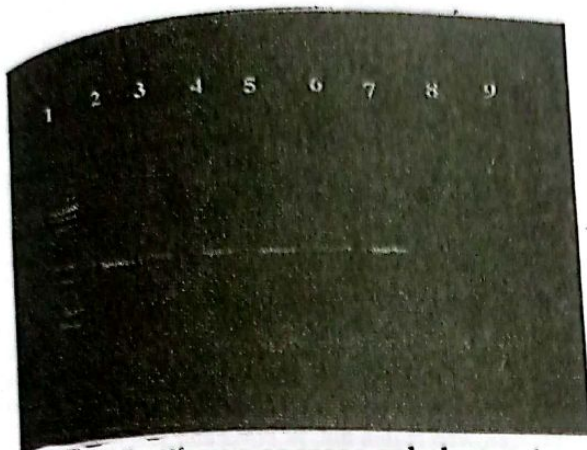
Photo. (4): Shows agarose gel electrophoresis showing amplification of 928 bp fragment of M. bovis genitalium
