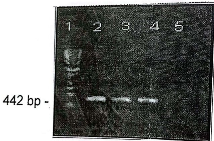
Photo. (3): Shows agarose gel electrophoresis showing amplification of 442 bp fragment of M. bovis
