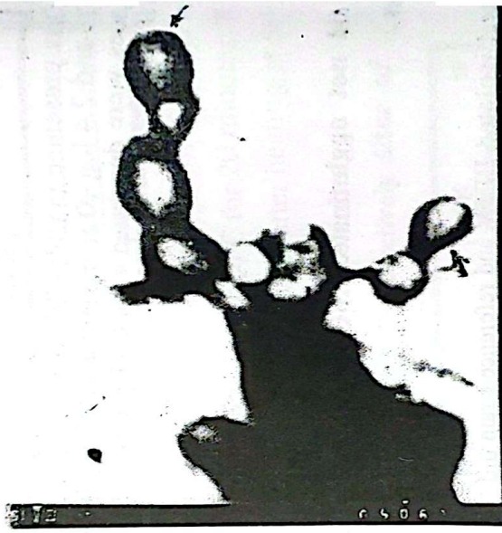
(2) Electron micrographs of BEFV stained with 4% ammonium molybdate X80.000 (bullet, cone shape, Truncated cone shaped particles).
