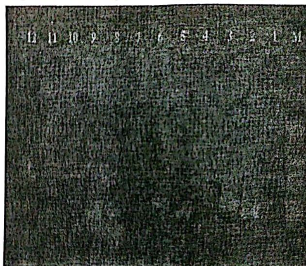
Fig.(1) agarose gel electrophoresis of multiplex PCR amplified products.
